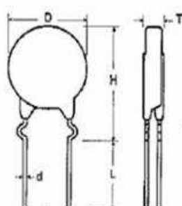
C Type(Out Crimped Lead)
