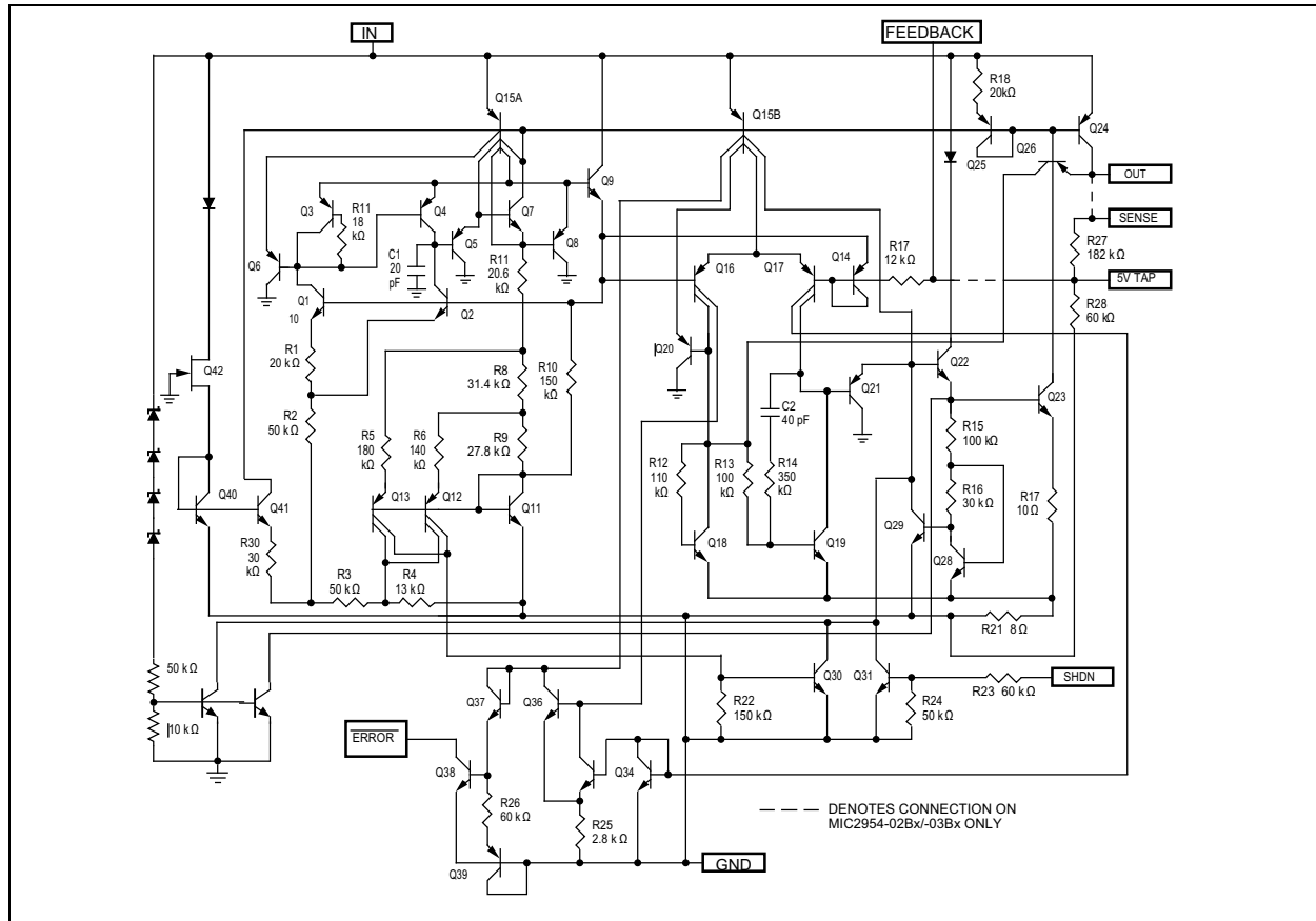
FIGURE 4-3: Schematic Diagram.
