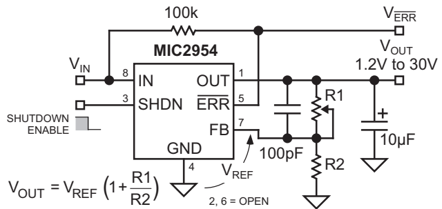
MIC2954 ADJUSTABLE REGULATOR
